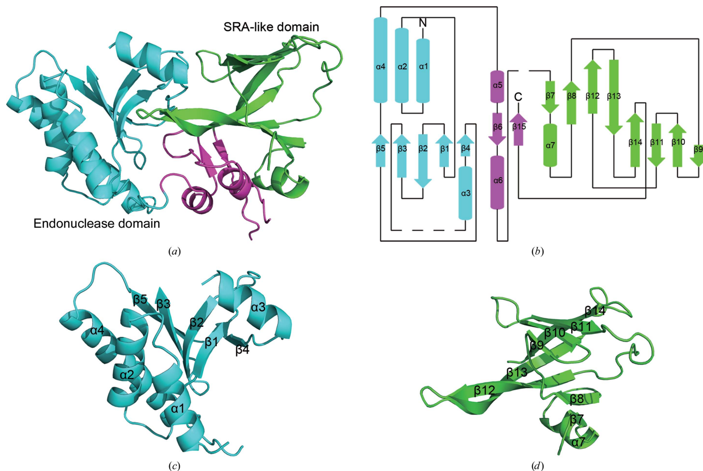
Figure 1 Overall structure of PvuRts1I. (a) Ribbon representation of PvuRts1I. The endonuclease domain and SRA-like domain are coloured cyan and green, respectively. (b) Schematic drawing of the topology of PvuRts1I. (c) Ribbon representation of the N-terminal endonuclease domain of PvuRts1I. (d) Ribbon representation of the C-terminal SRA-like domain of PvuRts1I.
