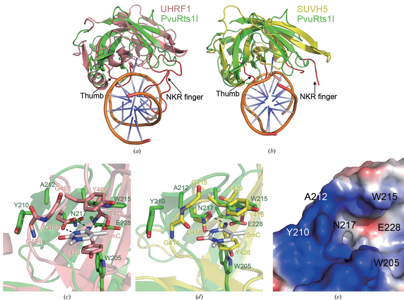
Figure 4 The putative substrate-recognition site of PvuRts1I. Comparison of the SRA-like domain structure of PvuRts1I (green) with the SRA-domain structure of (a) human UHRF1 (PDB entry 3clz, pink; Avvakumov et al. , 2008) and (b) Arabidopsis SUVH5 (PDB entry 3q0f, yellow; Rajakumara et al. , 2011) in complex with substrate DNA. The NKR finger and thumb loop are coloured red and indicated by arrows. A detailed view of the putative 5-hmC binding pocket superimposed on the 5-mC binding pocket of (c) human UHRF1 and (d) Arabidopsis SUVH5. The amino-acid residues and 5-mC are shown in stick representation. (e) Surface representation of the SRA-like domain of PvuRts1I. Amino-acid residues proposed to be involved in 5-hmC recognition are labelled.
