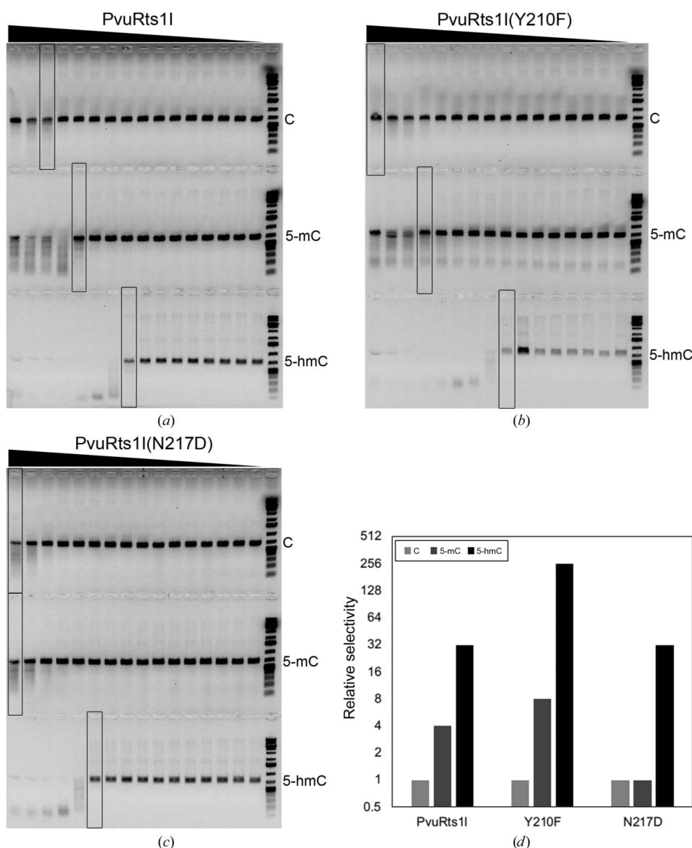
Figure 6 Relative selectivity of PvuRts1I and enzyme variants on unmodified cytosine (C), 5-mC and 5-hmC (see §2 for a description of the methods used). In each gel, the amount of enzyme is titrated from left (high) to right (low). All DNA substrates were made by PCR. (a) PvuRts1I; the approximate relative selectivity is 5-hmC:5-mC:C = 32:4:1. (b) Y210F mutant; the approximate relative selectivity is 5-hmC:5-mC:C = 256:8:1. (c) N217D mutant; the approximate relative selectivity is 5-hmC:5-mC:C = 32:1:1. (d) Comparison of the relative selectivity towards 5-hmC, 5-mC and C for PvuRts1I and the Y210F and N217D mutants. The relative selectivity is plotted on a log scale and normalized based on the activity of C.
