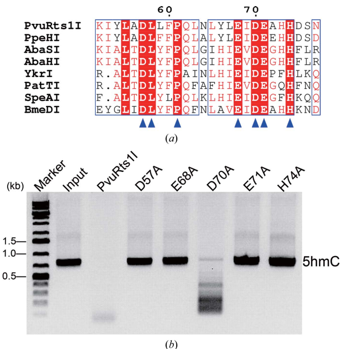
Figure 2 The conserved putative motif of the nuclease domain of PvuRts1I that is involved in metal-ion binding and catalysis. (a) Sequence alignment of the putative motif of PvuRts1I homologues. Absolutely conserved amino acids are indicated by blue triangles. (b) The in vitro modification-dependent enzymatic activity of PvuRts1I and its mutants on 5-hmC.
