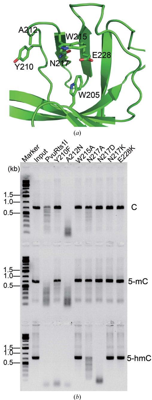
Figure 5 Improving the substrate selectivity of PvuRts1I via point mutations (see §2 for a description of the methods used). (a) Detailed view of the SRA-like domain of PvuRts1I. Amino acids potentially involved in the recognition of 5-hmC are shown in stick mode. (b) Endonuclease activity of PvuRts1I and its mutants towards C (cytosine; upper panel), 5-mC (5-methylcytosine; middle panel) and 5-hmC (5-hydroxymethylcytosine; bottom panel).
